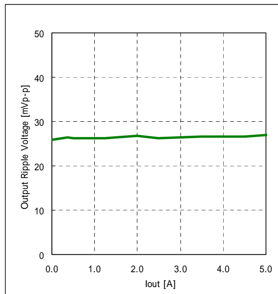
Fig.7-1-9. Ripple Voltage v.s. Output Current
