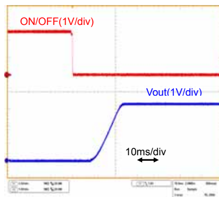
Fig.7-2-10. Start-up Waveform( I_o=5A )
