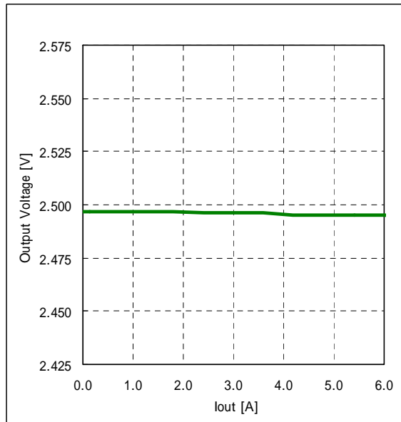
Fig.7-1-4. Output Voltage v.s. Output Current
