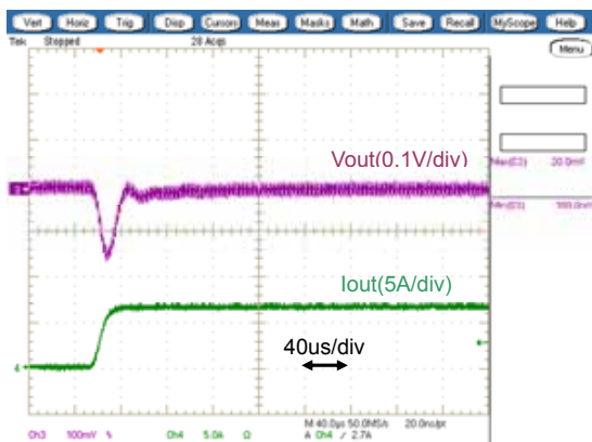
Fig.7-2-7. Load Transient Response ( I_o=0 6A)
