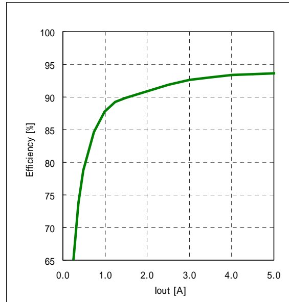
Fig.7-1-11. Efficiency v.s. Output Current
