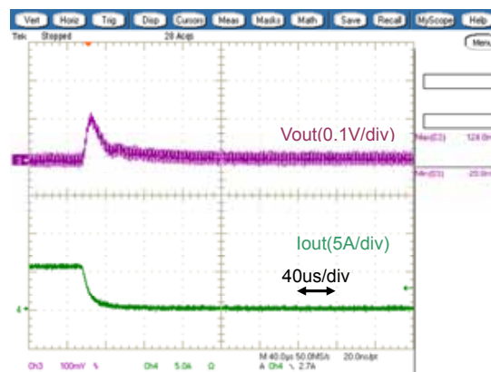
Fig.7-2-12. Load Transient Response ( I_o=5A 0A)
