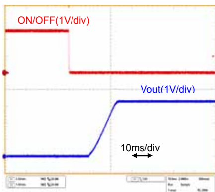
Fig.7-2-9. Start-up Waveform( I_o=0A )
