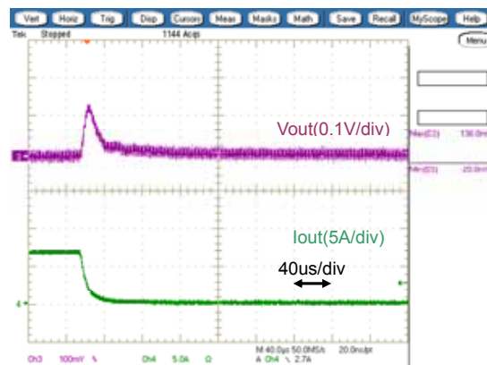
Fig.7-2-8. Load Transient Response ( I_o=6A 0A)
