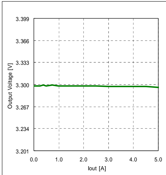
Fig.7-1-10. Output Voltage v.s. Output Current
