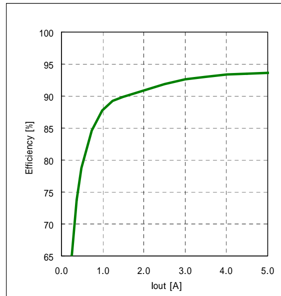
Fig.7-1-8. Efficiency v.s. Output Current
