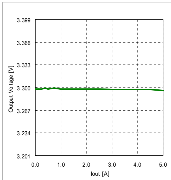
Fig.7-1-7. Output Voltage v.s. Output Current
