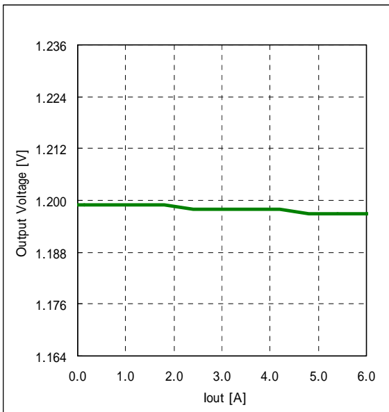
Fig.7-1-1. Output Voltage v.s. Output Current
