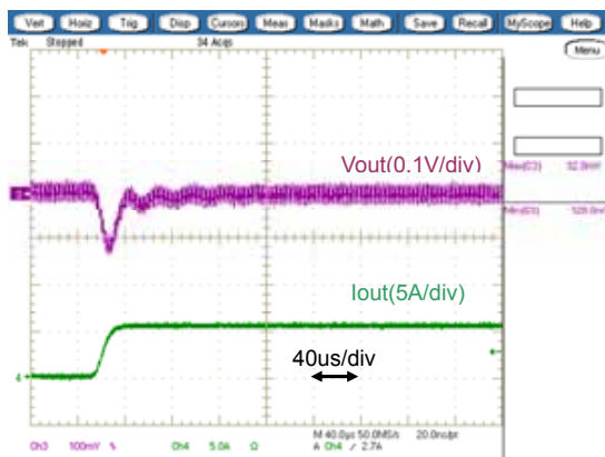
Fig.7-2-15. Load Transient Response ( I_o=0 5A)
