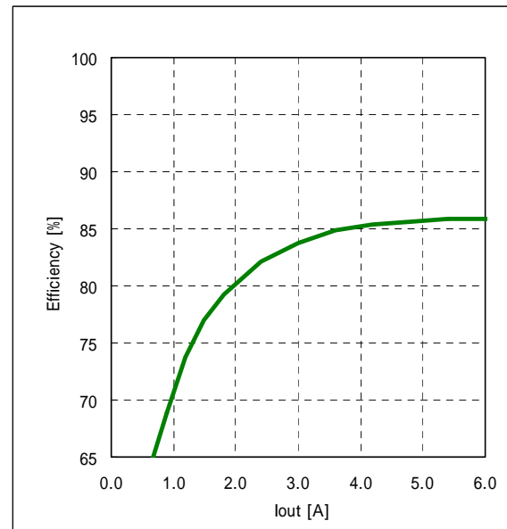
Fig.7-1-2. Efficiency v.s. Output Current
