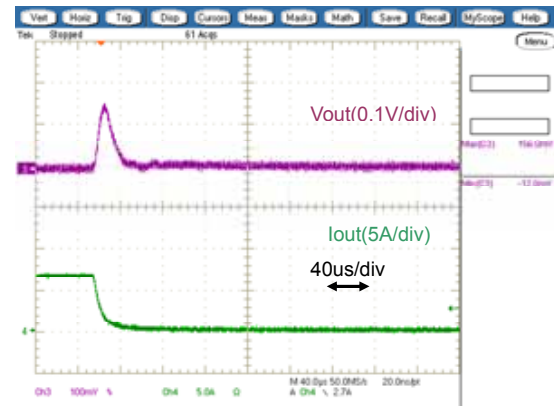
Fig.7-2-4. Load Transient Response ( I_o=6A 0A)
