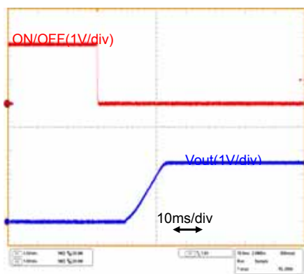
Fig.7-2-5. Start-up Waveform( I_o=0A )
