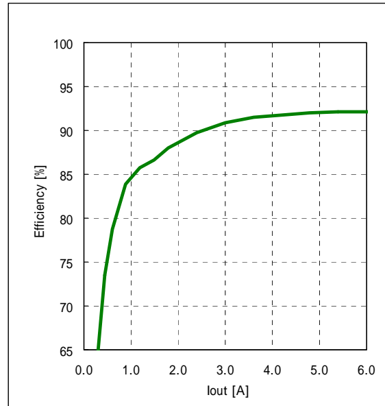
Fig.7-1-5. Efficiency v.s. Output Current
