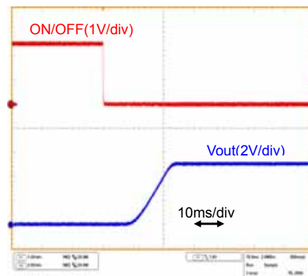
Fig.7-2-14. Start-up Waveform( I_o=5A )
