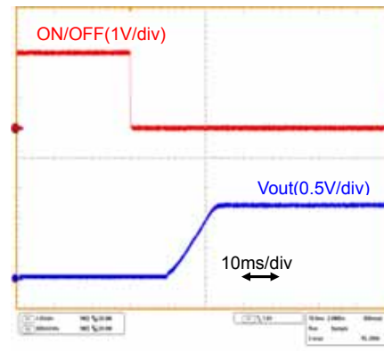
Fig.7-2-2. Start-up Waveform( I_o=6A )
