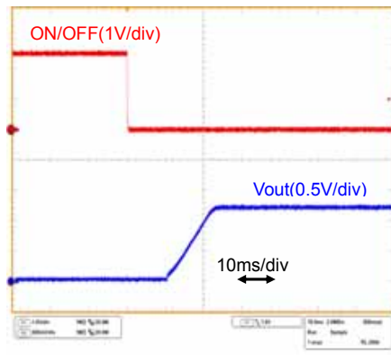
Fig.7-2-1. Start-up Waveform( I_o=0A )
