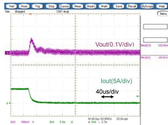
Fig.7-2-16. Load Transient Response ( I_o=5A 0A)
