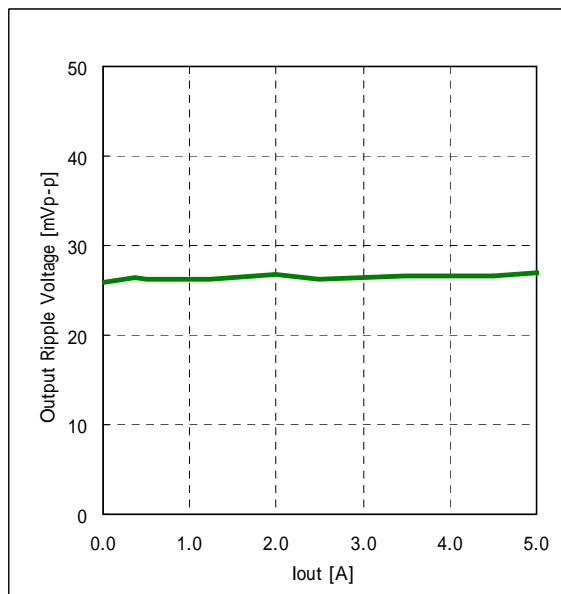
Fig.7-1-12. Ripple Voltage v.s. Output Current
