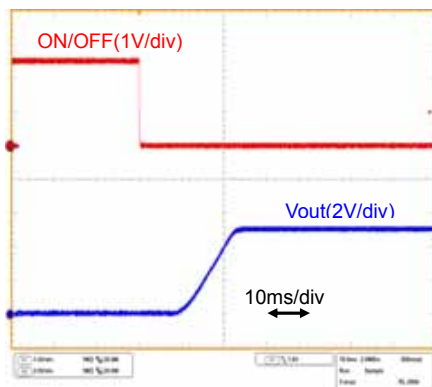
Fig.7-2-13. Start-up Waveform( I_o=0A )
