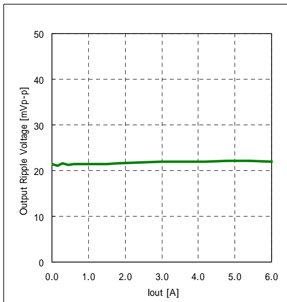
Fig.7-1-6. Ripple Voltage v.s. Output Current
