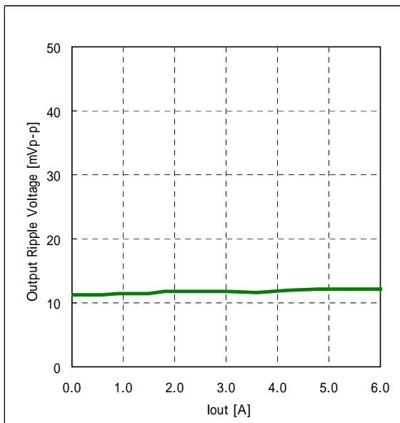
Fig.7-1-3. Ripple Voltage v.s. Output Current
