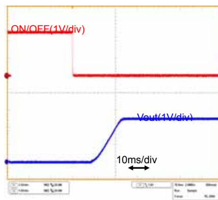
Fig.7-2-6. Start-up Waveform( I_o=6A )
