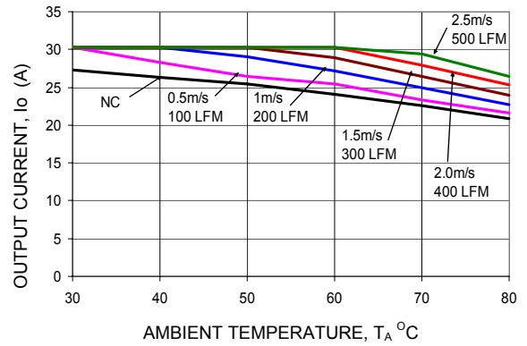
Figure 22. Output Current Derating versus Ambient Temperature and Airflow (ATM030A0X3-SR).
