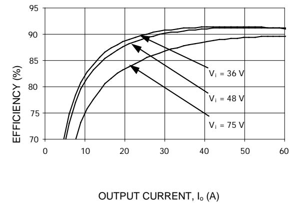
Figure 14. Converter Efficiency Vs Load at Room temperature.
