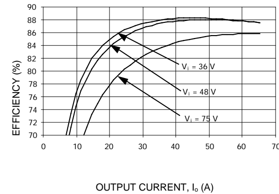
Figure 26. Converter Efficiency Vs Load at Room temperature.
