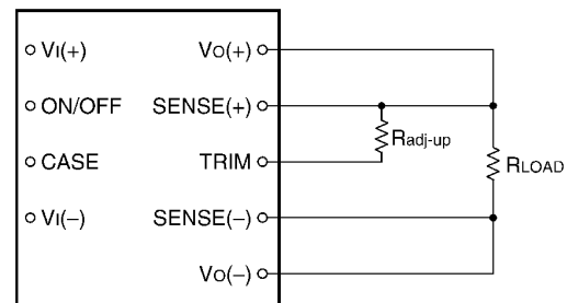
Figure 49. Circuit Configuration to Increase Output Voltage.
