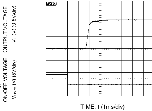
Figure 40. Typical Start-Up Characteristics from Remote ON/OFF.
