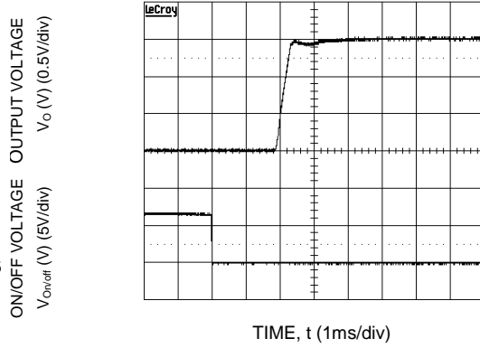
Figure 34. Typical Start-Up Characteristics from Remote ON/OFF.
