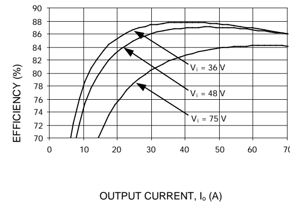
Figure 32. Converter Efficiency Vs Load at Room temperature.
