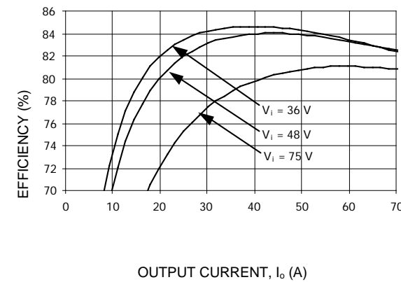
Figure 38. Converter Efficiency Vs Load at Room temperature.
