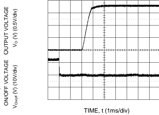
Figure 28. Typical Start-Up Characteristics from Remote ON/OFF.
