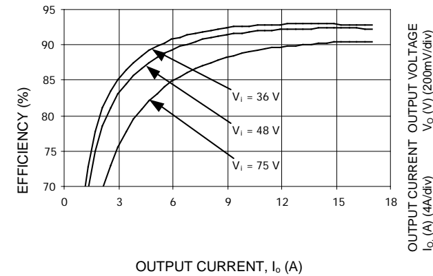
Figure 2. Converter Efficiency Vs Load at Room temperature.
