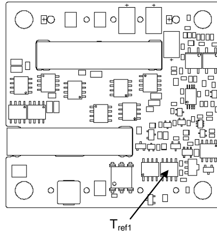
Figure 51. T_{ref} Temperature Measurement Location for V_o= 5V .
