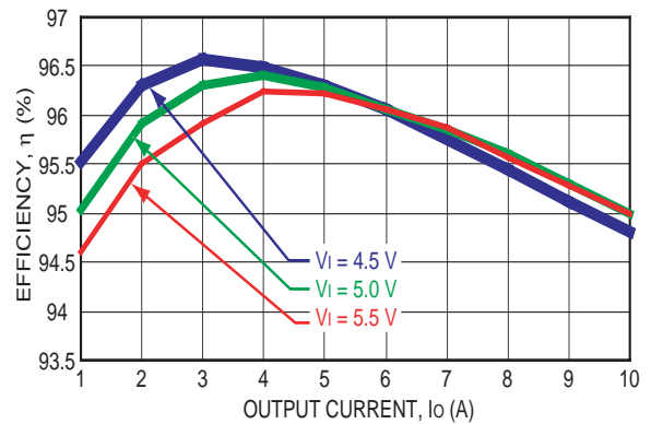
Figure 10. Converter Efficiency vs Output Current AXH010A0F (3.3V Output Voltage).
