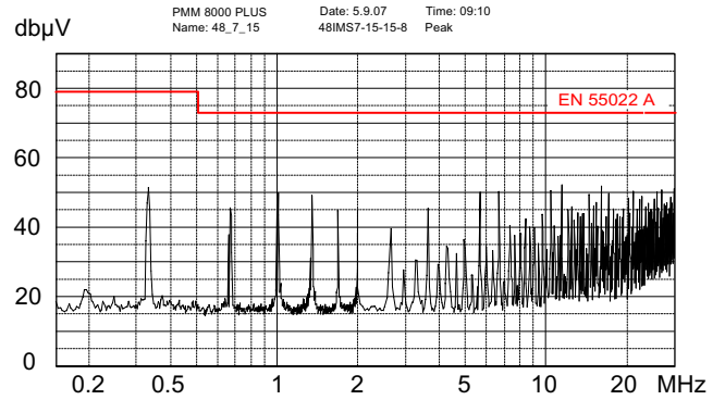
Fig. 17 48IMS7-15-15-8: Typical conducted emissions (peak) at the input at V_{i\text{nom}} and I_{o\text{nom}} according to EN 55011/22. Output leads 0.1 m, twisted. External input capacitor (1 \mu\text{F} ceramic + 47 \mu\text{F} electrolytic cap).
