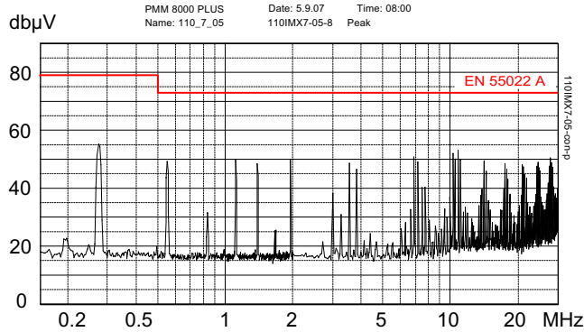
Fig. 16c 110IMX7-05-8: Typical conducted emissions (peak) at the input at V_{i\text{nom}} and I_{o\text{nom}} according to EN 55011/22. Output leads 0.1 m, twisted. External input capacitor (0.15 \mu\text{F} ceramic + 4.7 \mu\text{F} electrolytic cap).
