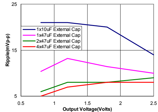
Figure 49. Output ripple voltage for various output voltages with external 1x10 μF, 1x47 μF, 2x47 μF or 4x47 μF ceramic capacitors at the output (30A load). Input voltage is 5V.
