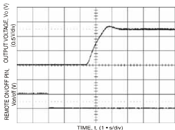
Figure 6. Start-up from Remote On/Off ( I_O = I_{O, \text{max}} ).
