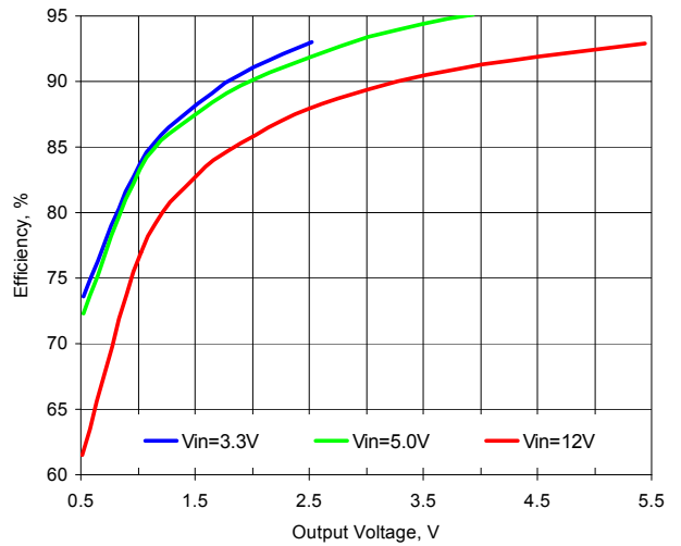
Figure 5. Efficiency vs. Output Voltage, Iout=20A, Fsw=500kHz
