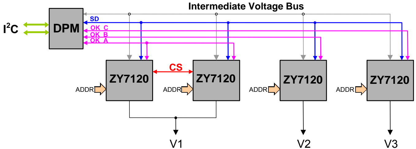
Figure 25. Block Diagram of Typical Multiple Output Application with Digital Power Manager and I 2 C Interface
