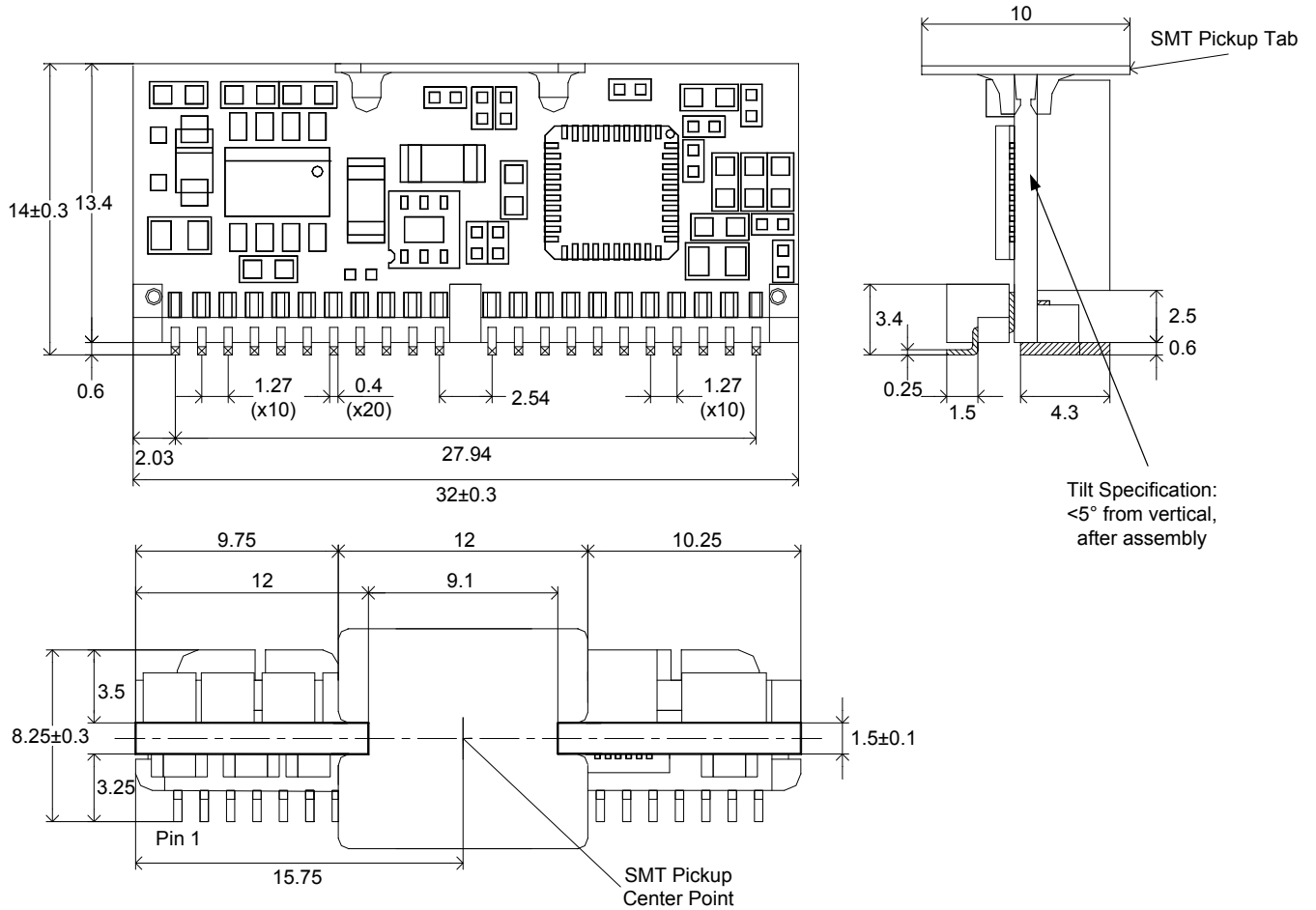
Figure 58. Mechanical Drawing
