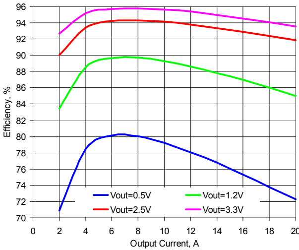
Figure 3. Efficiency vs. Load. Vin=5V, Fsw=500kHz
