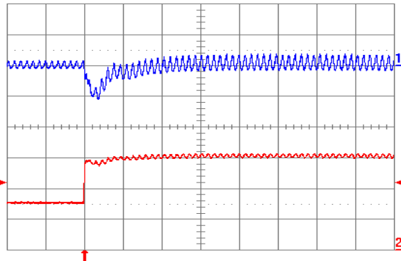
Fig. 1.2V.6: Output voltage response for V_{out} = 1.2 V to positive load current step change from 2.5 A to 5 A with slew rate of 5 A/ \mu\text{s} at V_{in} = 5 V. Top trace: output voltage (100 mV/div.); Bottom trace: load current (2 A/div.). C_o = 47 \mu\text{F} ceramic + 1 \mu\text{F} ceramic. Time scale: 20 \mu\text{s} /div.
