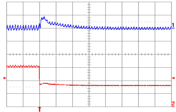
Fig. 0.7525V.8: Output voltage response for V_{out} = 0.7525 V to negative load current step change from 5 A to 2.5 A with slew rate of -5 \text{ A}/\mu\text{s} at V_{in} = 5 V. Top trace: output voltage (100 mV/div.); Bottom trace: load current (2 A/div.). C_o = 47 \mu\text{F} ceramic + 1 \mu\text{F} ceramic. Time scale: 20 \mu\text{s} /div.
