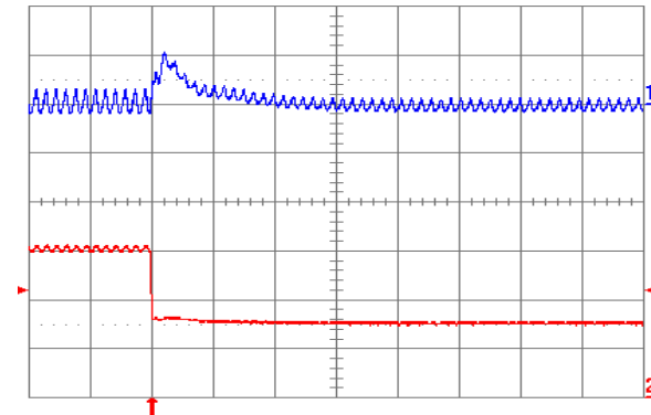
Fig. 1.2V.8: Output voltage response for V_{out} = 1.2 V to negative load current step change from 5 A to 2.5 A with slew rate of -5 A/ \mu\text{s} at V_{in} = 5 V. Top trace: output voltage (100 mV/div.); Bottom trace: load current (2 A/div.). C_o = 47 \mu\text{F} ceramic + 1 \mu\text{F} ceramic. Time scale: 20 \mu\text{s} /div.
