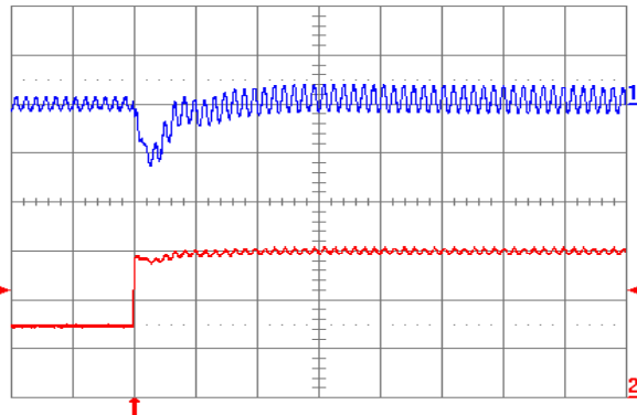
Fig. 1.8V.7: Output voltage response for V_{out} = 1.8\text{ V} to positive load current step change from 2.5\text{ A} to 5\text{ A} with slew rate of 5\text{ A}/\mu\text{s} at V_{in} = 5\text{ V} . Top trace: output voltage ( 100\text{ mV/div.} ); Bottom trace: load current ( 2\text{ A/div.} ). C_o = 47\text{ }\mu\text{F} ceramic + 1\text{ }\mu\text{F} ceramic. Time scale: 20\text{ }\mu\text{s/div.}
