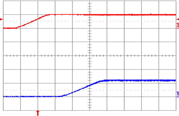
Fig. 1.2V.5: Turn-on transient for V_{out} = 1.2 V with application of V_{in} at full rated load current (resistive) and 47 \mu\text{F} external capacitance at V_{in} = 5 V. Top trace: V_{in} (5 V/div.); Bottom trace: output voltage (1 V/div.); Time scale: 2 ms/div.
