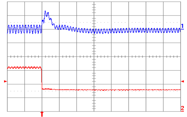
Fig. 2.5V.8: Output voltage response for V_{out} = 2.5 V to negative load current step change from 5 A to 2.5 A with slew rate of -5 A/ \mu\text{s} at V_{in} = 5 V. Top trace: output voltage (100 mV/div.); Bottom trace: load current (2 A/div.). C_o = 47 \mu\text{F} ceramic + 1 \mu\text{F} ceramic. Time scale: 20 \mu\text{s} /div.
