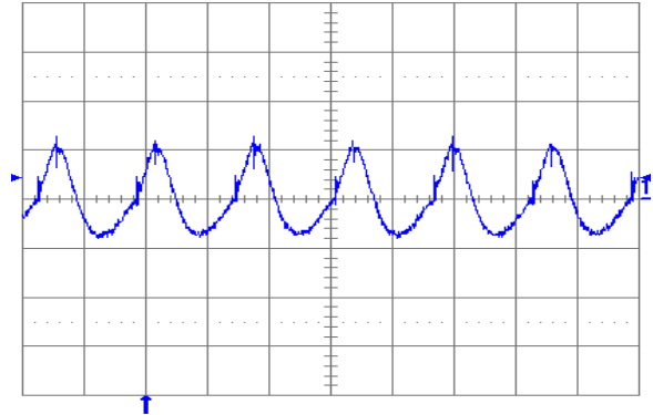
Fig. 0.7525V.5: Output voltage ripple (20 mV/div.) at full rated load current into a resistive load with external capacitance 10 \mu\text{F} ceramic + 1 \mu\text{F} ceramic and V_{in} = 5 V for V_{out} = 0.7525 V. Time scale: 2 \mu\text{s} /div.
