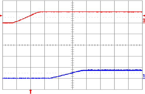
Fig. 0.7525V.4: Turn-on transient for V_{out} = 0.7525 V with application of V_{in} at full rated load current (resistive) and 47 \mu\text{F} external capacitance at V_{in} = 5 V. Top trace: V_{in} (5 V/div.); Bottom trace: output voltage (1 V/div.); Time scale: 2 ms/div.
