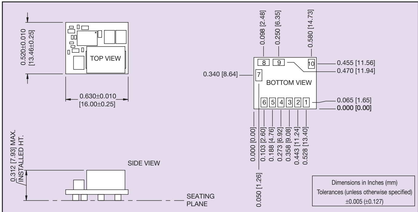
Figure 5 - Mechanical Drawing
