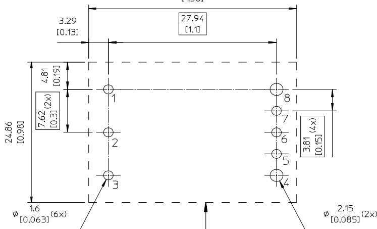
RECOMMENDED FOOTPRINT - TOP VIEW 34.52 [1.36]
