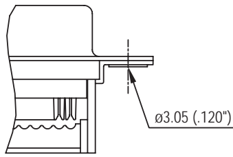
Standard rivet \varnothing 3.05mm no digit
