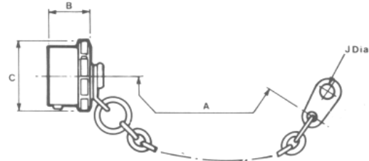
Caps and Chains Ribbed for Plugs
