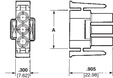
Plug Front
