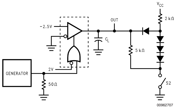
FIGURE 3. t_{ZL} , t_{LZ} (Notes 10, 11, 13, 14)
