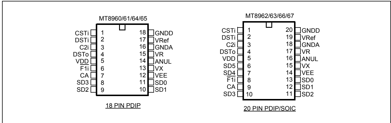
Figure 2 - Pin Connections
