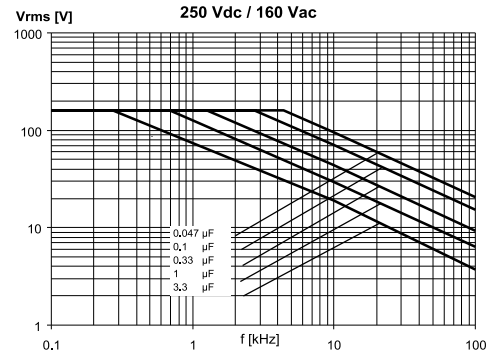
250 Vdc / 160 Vac
