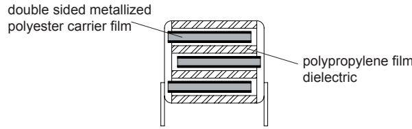
1 section (250Vdc)
