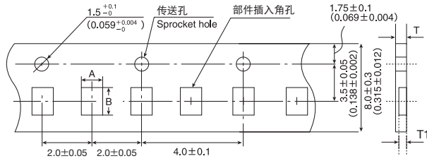
③ 编带尺寸 Taping dimensions 纸带 Paper Tape (8mm宽) (0.315inches wide)
