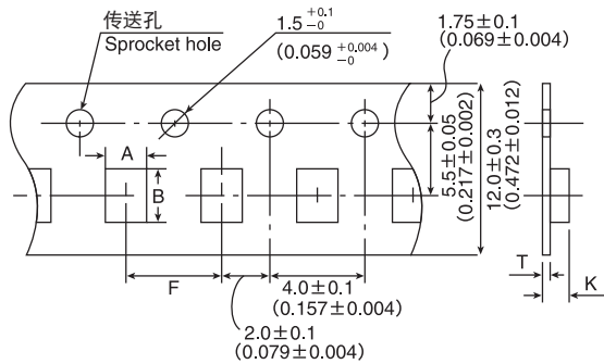
压印带 Embossed tape (12mm宽) (0.472inches wide)
