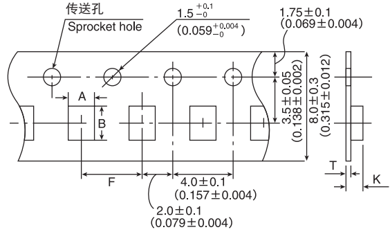
压印带 Embossed tape (8mm宽) (0.315inches wide)
