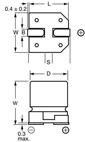
Fig.2 Dimensional outline
