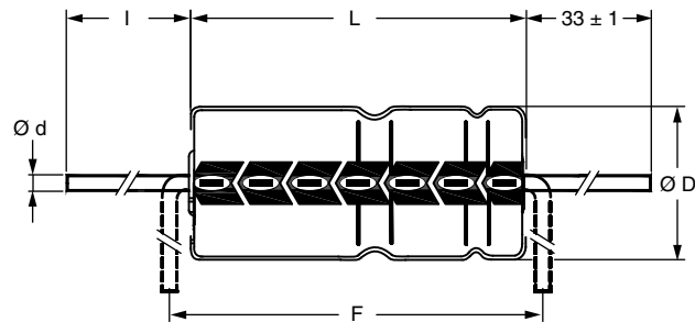
Form AA: Axial in box Case ∅ D x L = 10 mm x 30 mm to 21 mm x 38 mm
