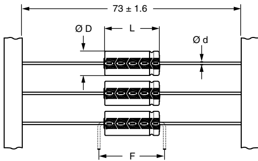
Form BR: Taped on reel Case ∅ D x L = 6.5 mm x 18 mm to 15 mm x 30 mm Form BA: Taped in box (ammopack) Case ∅ D x L = 6.5 mm x 18 mm to 10 mm x 25 mm
