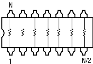
-3 Circuit - Isolated Resistors
