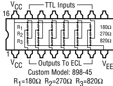
-45 Circuit - TTL to ECL Translator
