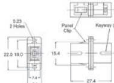
SC duplex coupling
