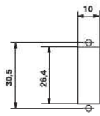
Hole pattern
