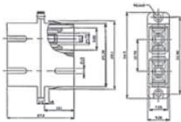
SC duplex coupling
