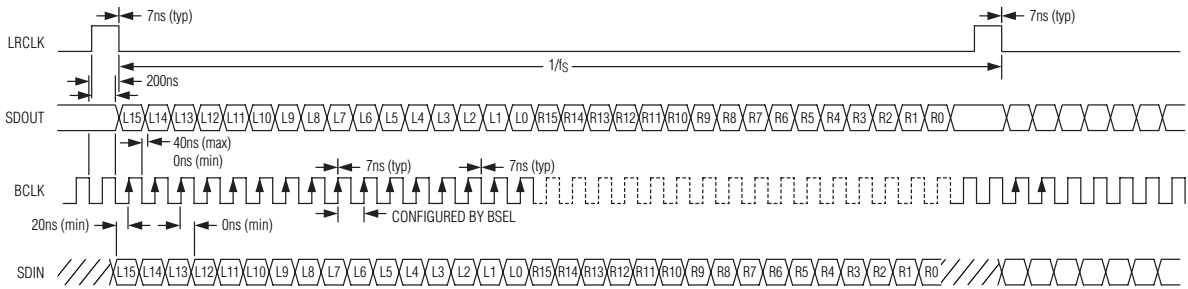
Figure 3. Digital Audio Interface Voice Master Mode
