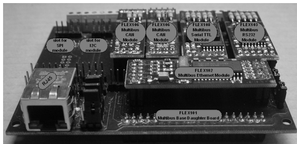
Figure 1: FLEX multibus pack
