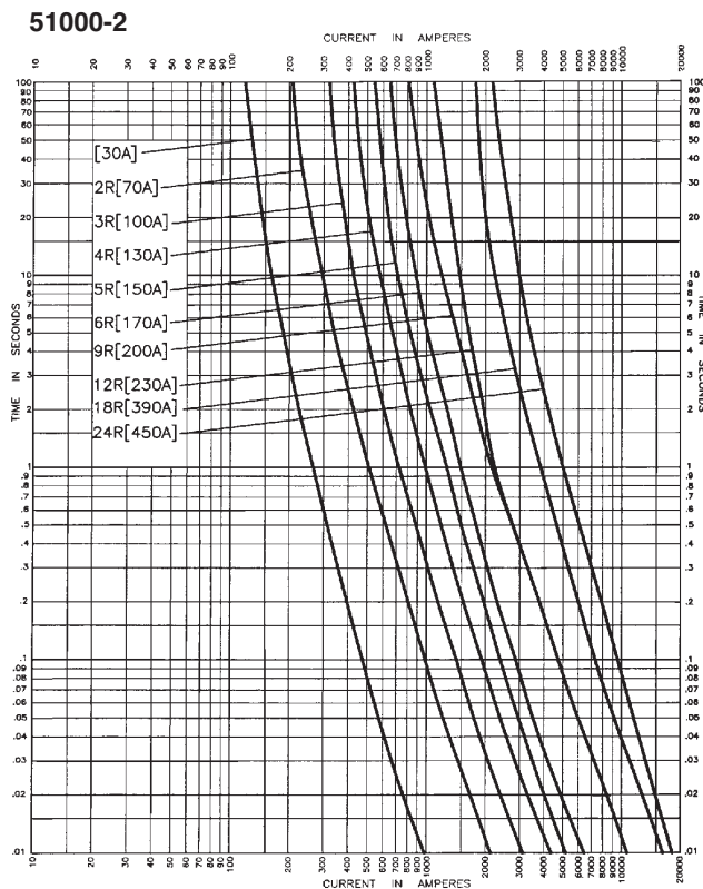
Time-Current Curve: Total Clearing
