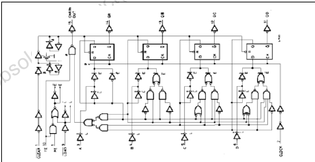
Figure 3: Logic Diagram
