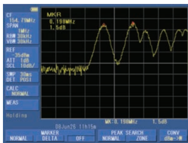
Delta marker measurement
