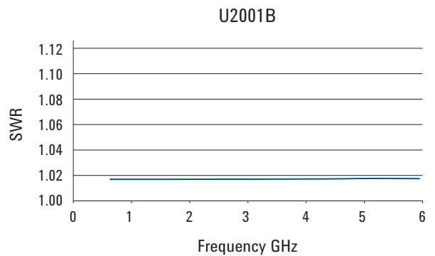
Typical SWR for U2001B sensor (25 °C ± 10 °C)
