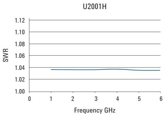
Typical SWR for U2001H sensor (25 °C ± 10 °C)
