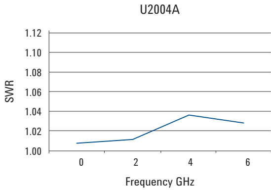
Typical SWR for U2004A sensor (25 °C ± 10 °C)
