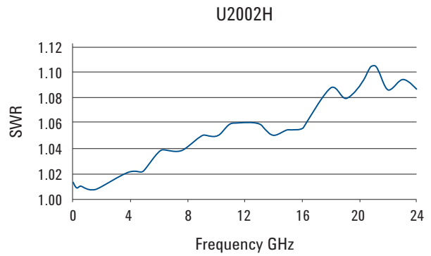
Typical SWR for U2002H sensor (25 °C ± 10 °C)
