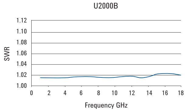
Typical SWR for U2000B sensor (25 °C ± 10 °C)
