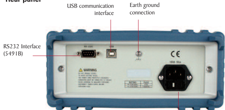
AC receptacle protected with I10/220V selectable line fuse
