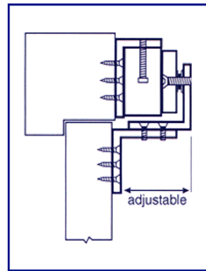
Z Bracket Installation Inward opening installation
