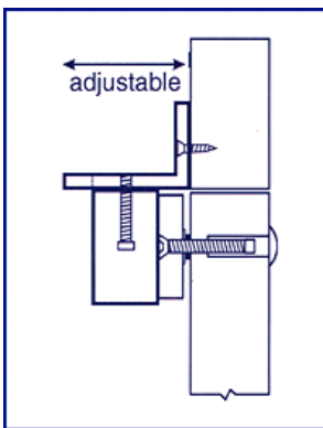
L Bracket Installation Outward opening installation
