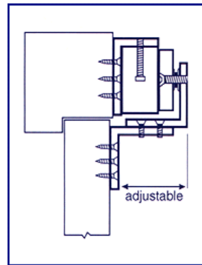
Z Bracket Installation Inward door installation
