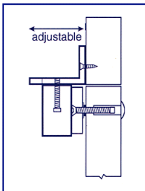
L Bracket Installation Outward door installation
