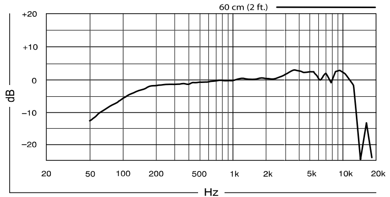
FREQUENCY RESPONSE
