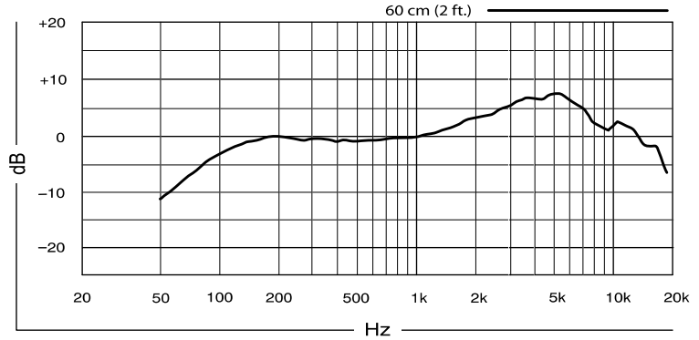
FREQUENCY RESPONSE
