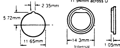
PANEL CUTOUT
