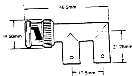
ORDER NO 251197 BNC PLUG TO (2) JACKS
