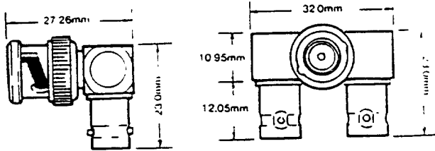
ORDER NO 251070 RIGHT ANGLE PLUG TO (2) JACKS
