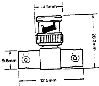
ORDER NO 251197 BNC PLUG TO (2) JACKS
