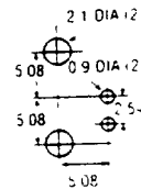
RIGHT ANGLE MOUNTING
