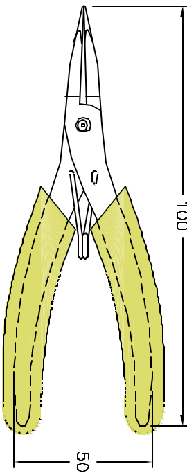
Micro round nose pliers
