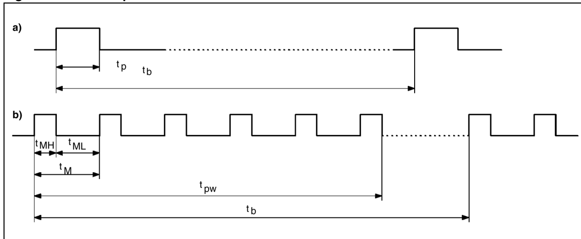
Figure 6. REMO Output Waveform
