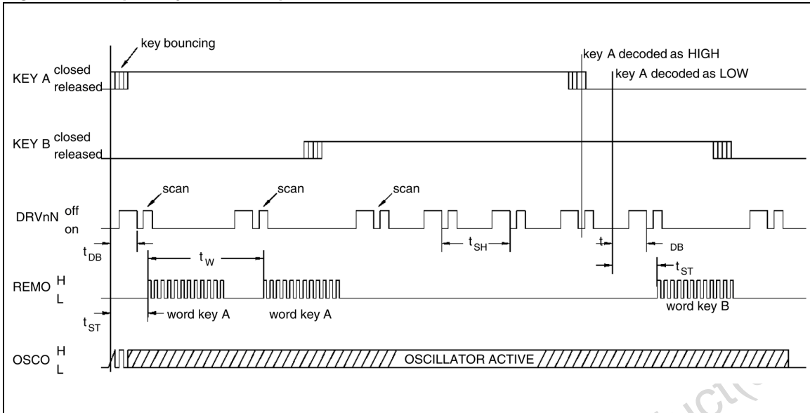
Figure 8. Multiple Key-Stroke Sequence
