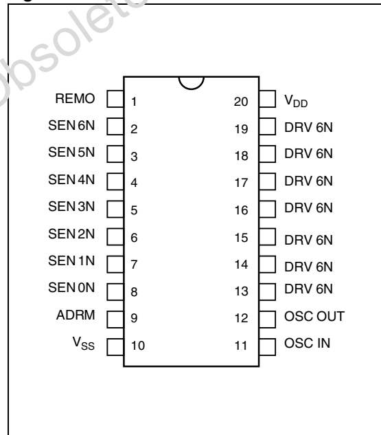
Figure 2. Pin Connection
