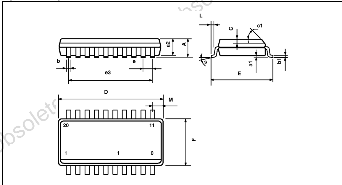
Figure 9. Package Dimensions
