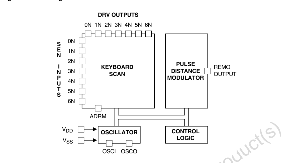
Figure 3. Block Diagram
