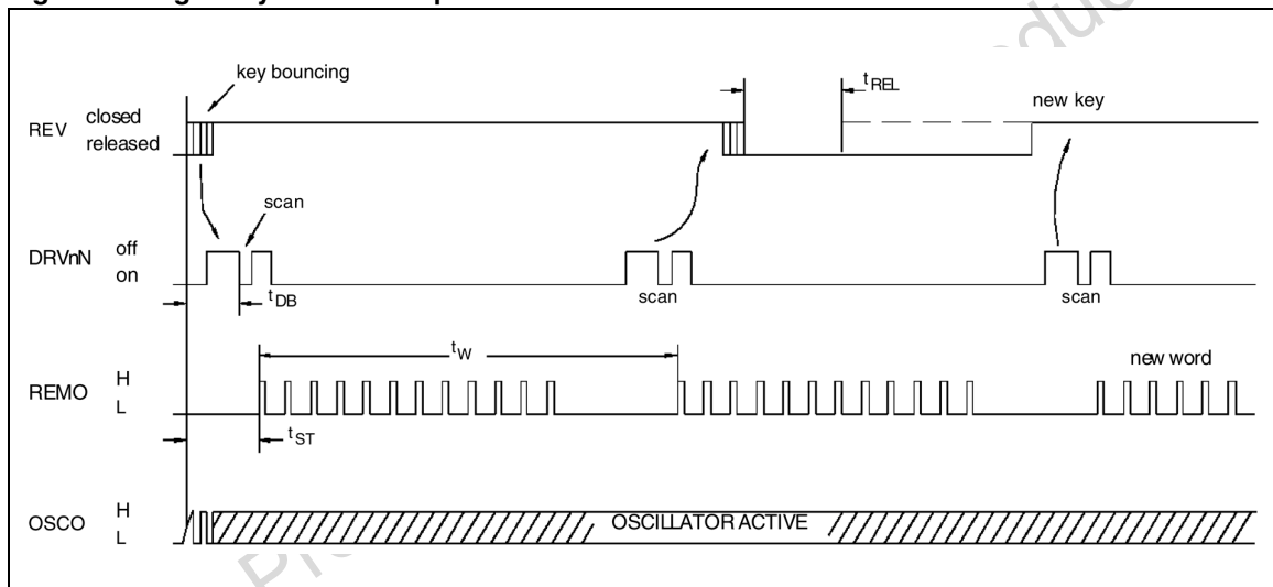
Figure 7. Single Key - Stroke Sequence
