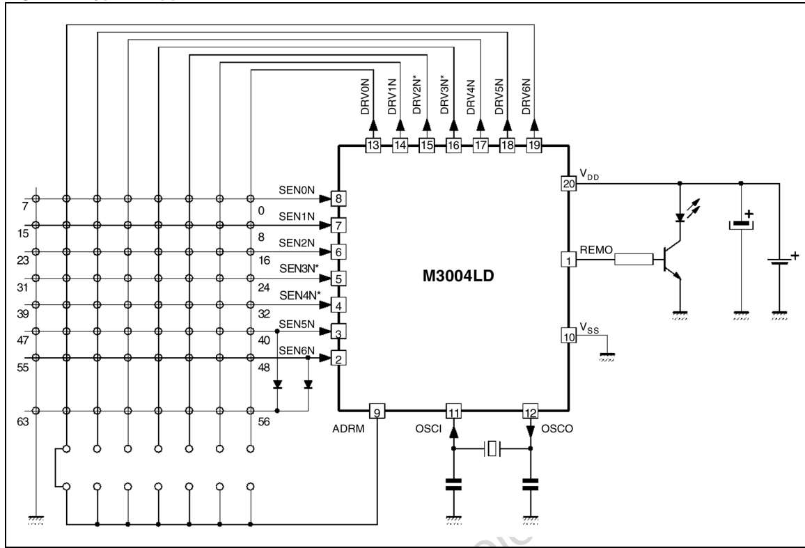
Figure 4. Typical Application
