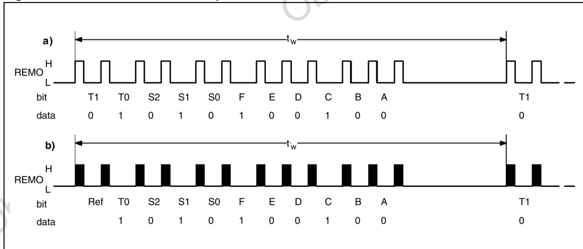
Figure 5. Data Format of REMO Output
