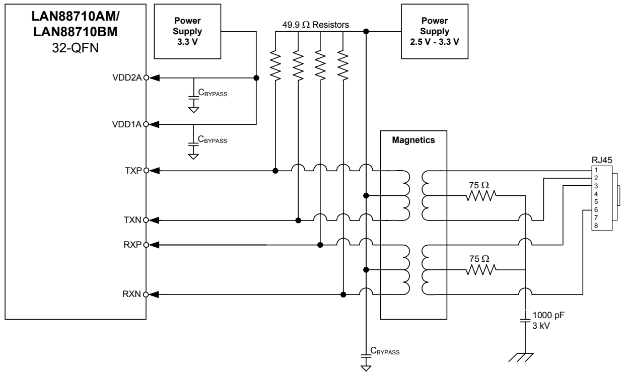
Figure 3.14 Twisted-Pair Interface Diagram (Dual Power Supplies)
