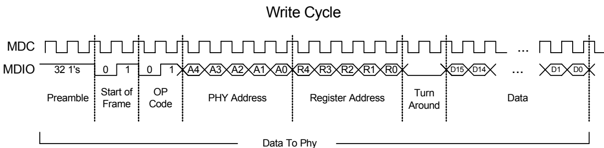
Figure 3.4 MDIO Timing and Frame Structure - WRITE Cycle
