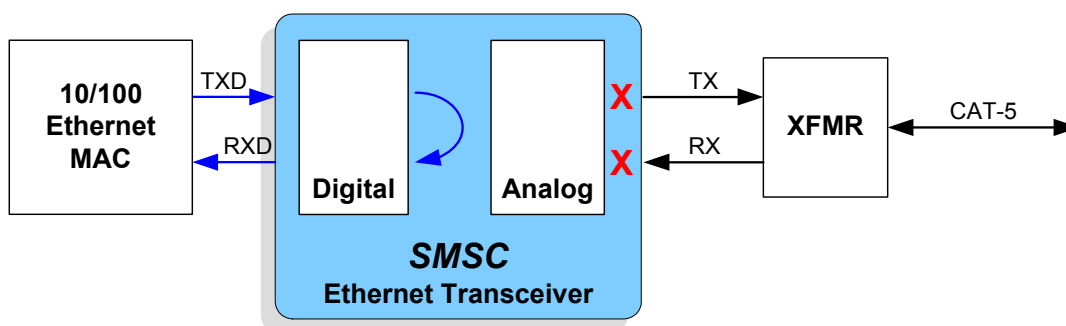
Figure 3.7 Near-end Loopback Block Diagram
