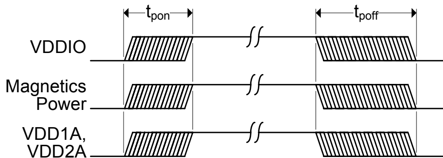
Figure 5.2 Power Sequence Timing
