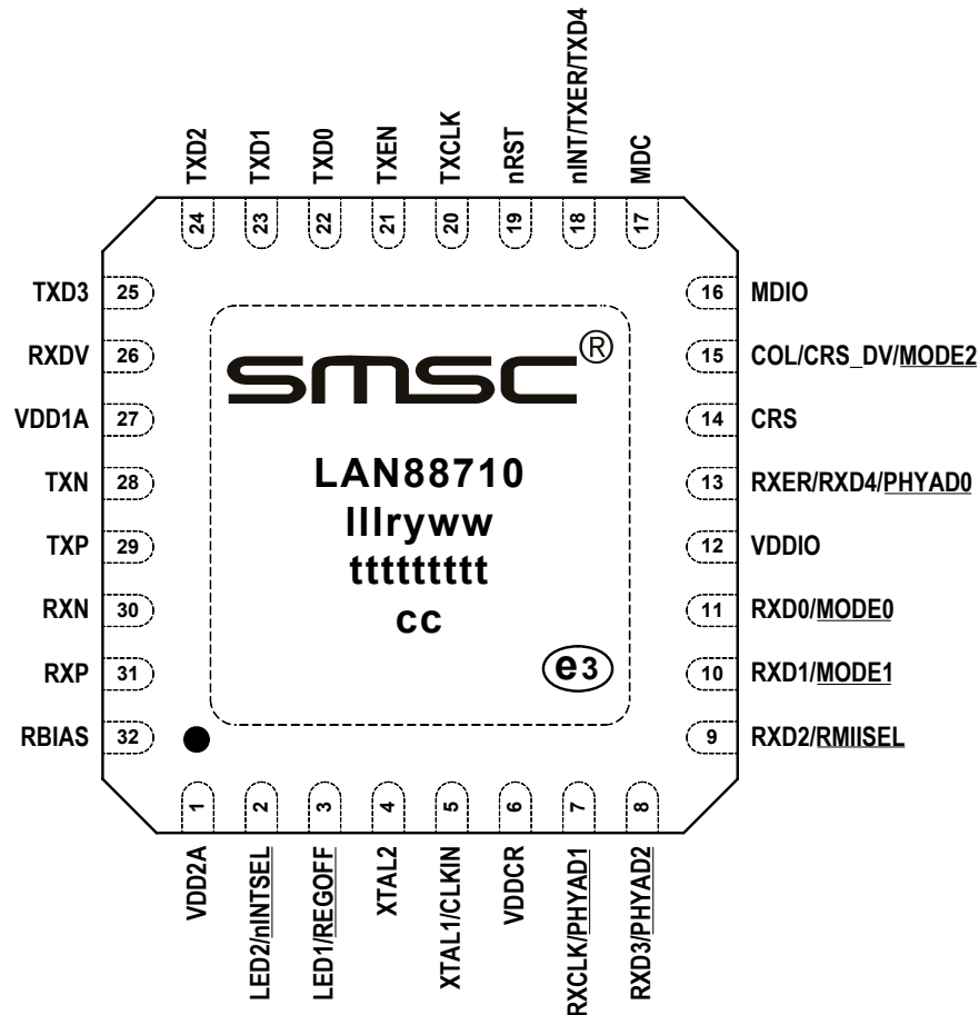
Figure 2.1 32-QFN Pin Assignments (TOP VIEW)
