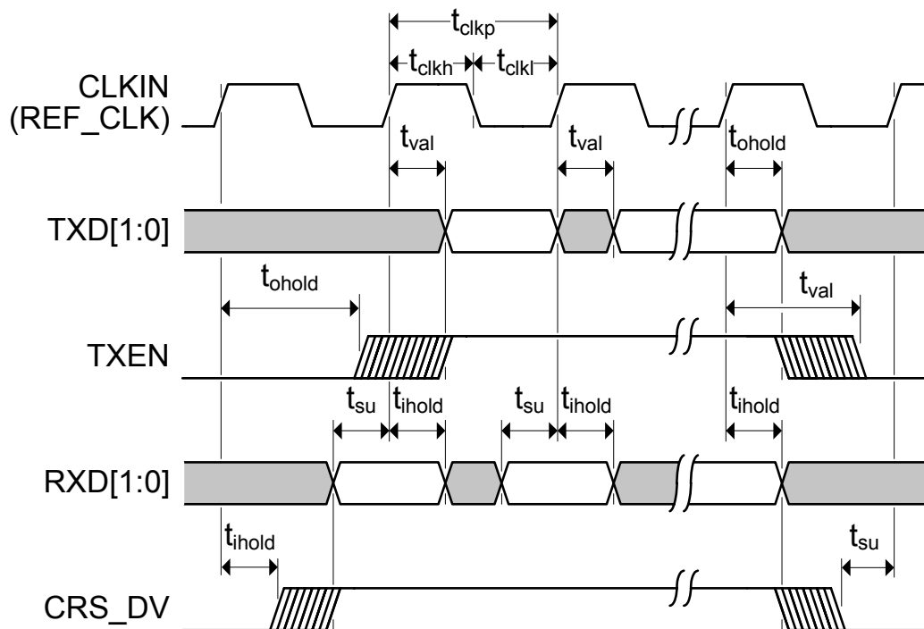
Figure 5.6 RMII Timing
