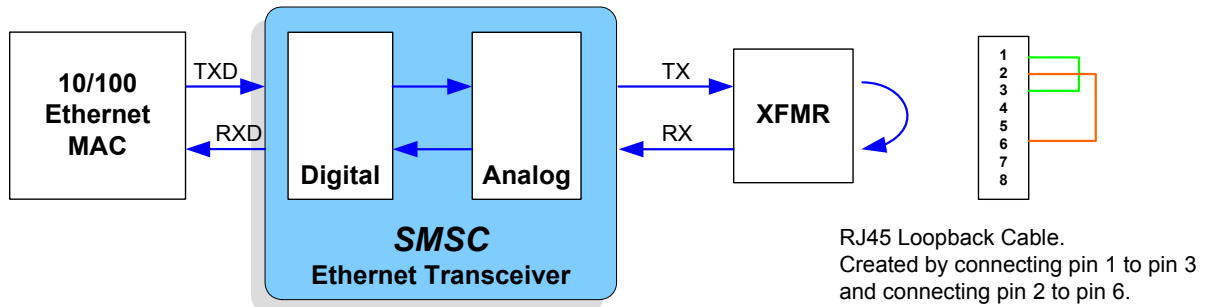
Figure 3.9 Connector Loopback Block Diagram
