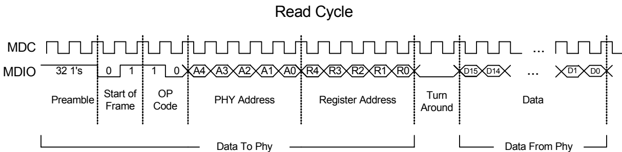
Figure 3.3 MDIO Timing and Frame Structure - READ Cycle
