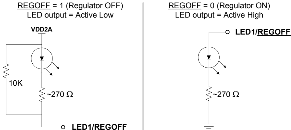
Figure 3.5 LED1/ REGOFF Polarity Configuration
