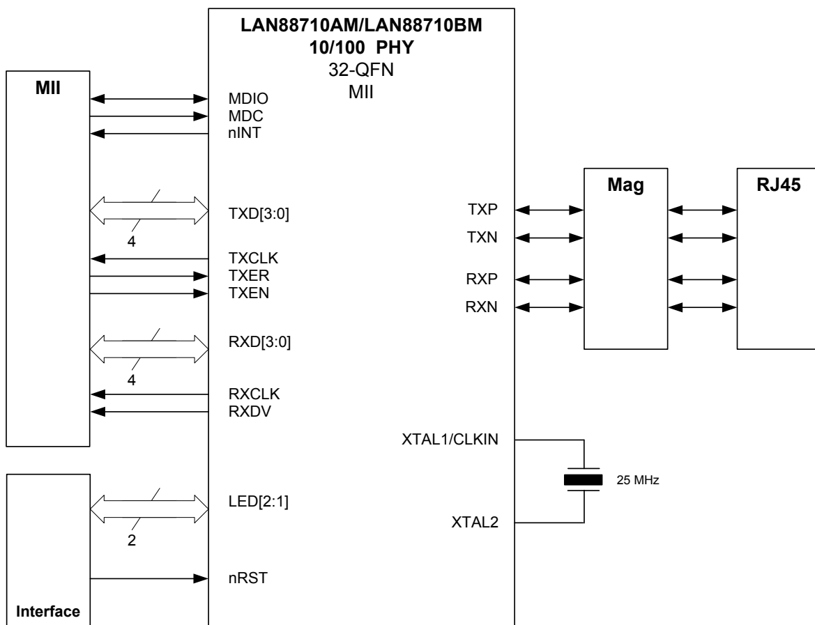
Figure 3.10 Simplified System Level Application Diagram
