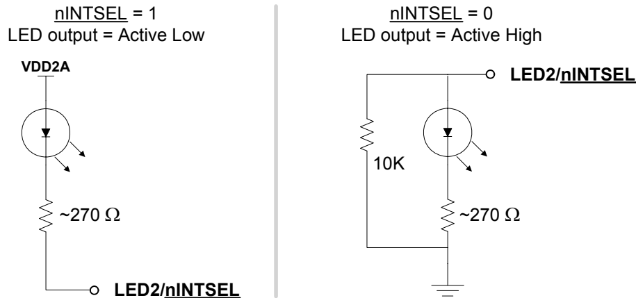
Figure 3.6 LED2/ nINTSEL Polarity Configuration
