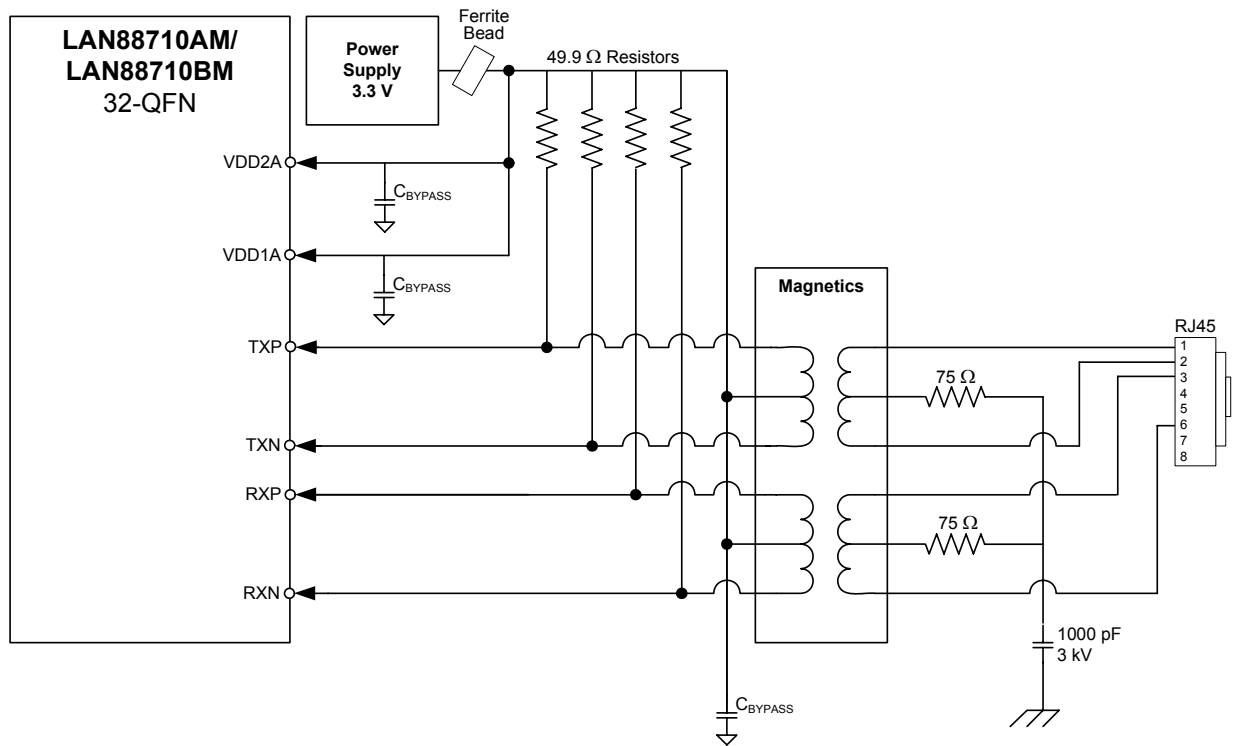
Figure 3.13 Twisted-Pair Interface Diagram (Single Power Supply)
