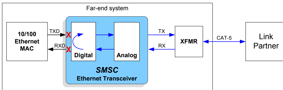
Figure 3.8 Far Loopback Block Diagram
