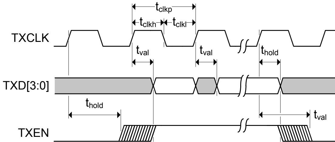
Figure 5.4 MII Transmit Timing
