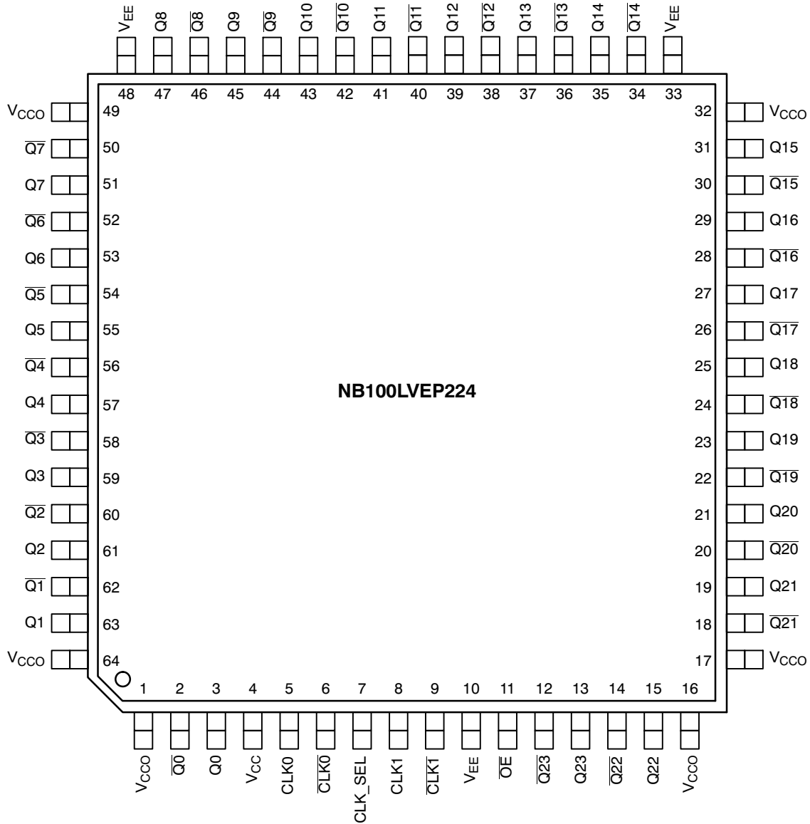
Figure 1. 64-Lead LQFP Pinout (Top View)
