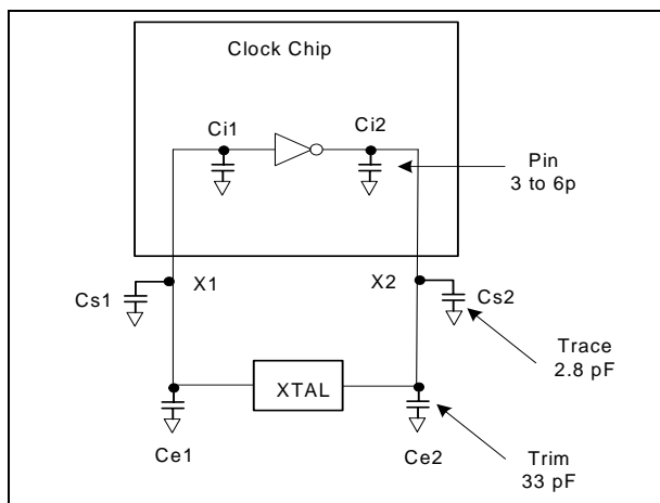
Figure 2. Crystal Loading Example
