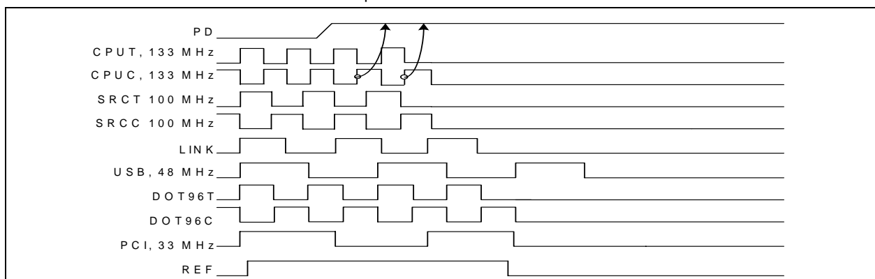
Figure 3. PD Assertion Timing Waveform
