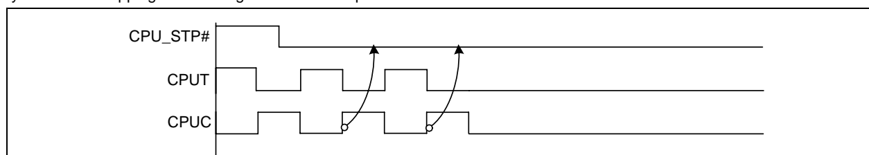
Figure 5. CPU_STP# Assertion Timing Waveform
