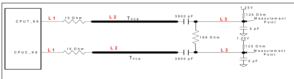
Figure 15. Differential Load Configuration for 0.7 Push Pull Clock
