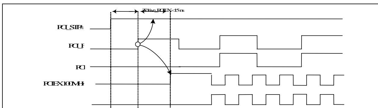
Figure 8. PCI_STP# Deassertion
