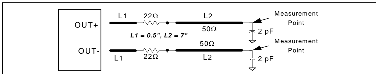
Figure 14. Differential Load Configuration for 0.7V Push Pull Clock
