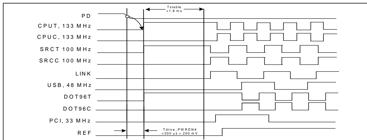
Figure 4. PD Deassertion Timing Waveform
