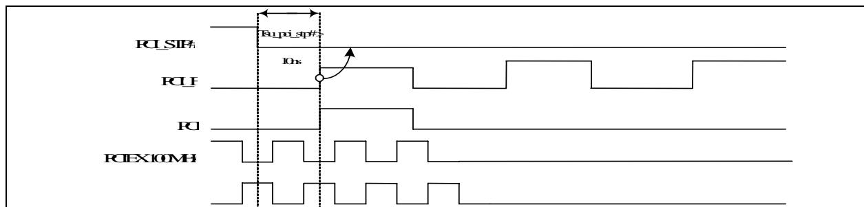
Figure 7. PCI_STP# Assertion
