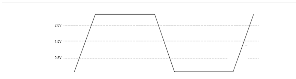
Figure 18. Single-ended Output Signals (for AC Parameters Measurement)
