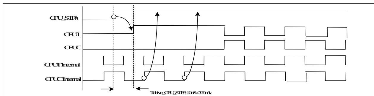
Figure 6. CPU_STP# Deassertion
