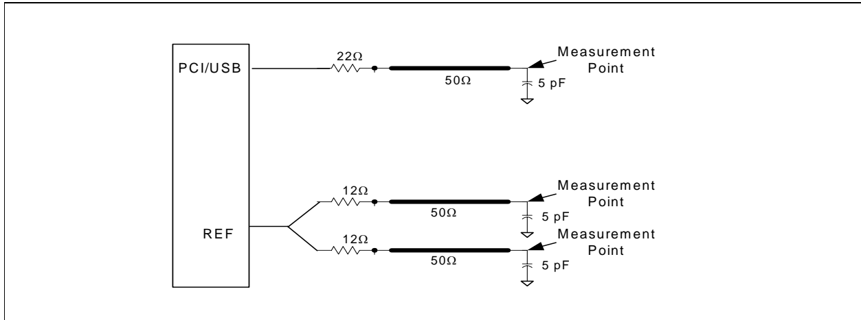
Figure 12. Single-ended Load Configuration
