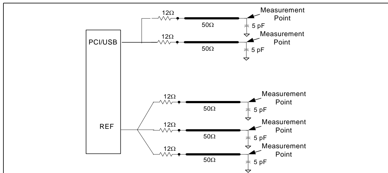
Figure 13. Single-ended Load Configuration HIGH DRIVE OPTION
