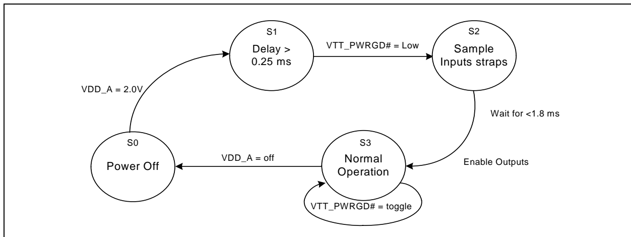
Figure 10. VTT_PWRGD# Timing Diagram
