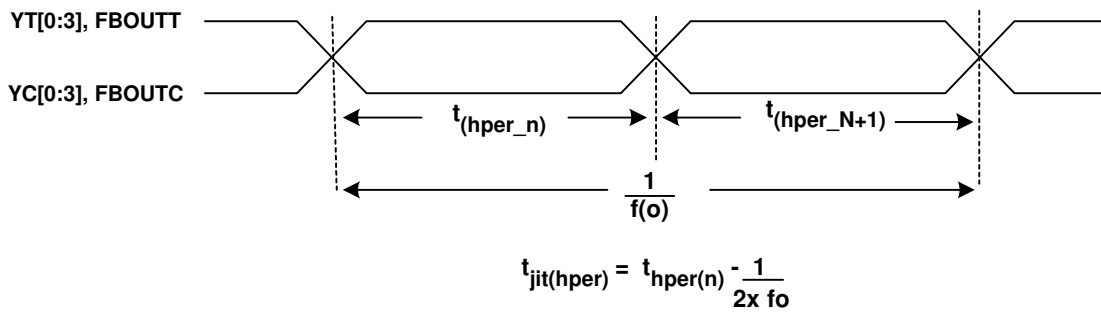
Figure 4. Half-period Jitter
