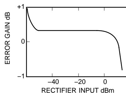
Figure 10. Rectifier Accuracy
