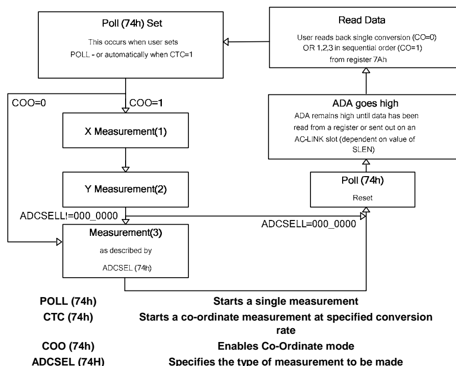
Figure 32 Touchpanel Conversion Flow Diagram
