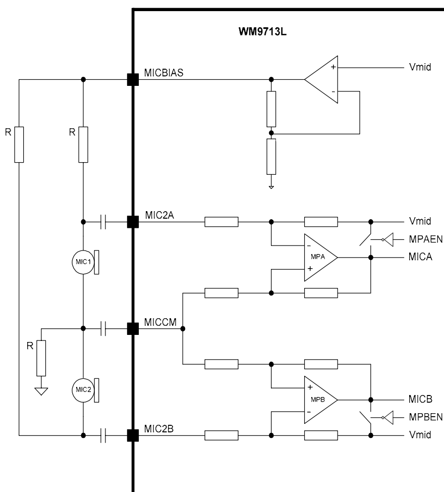
Figure 21 Dual Microphone Configuration
