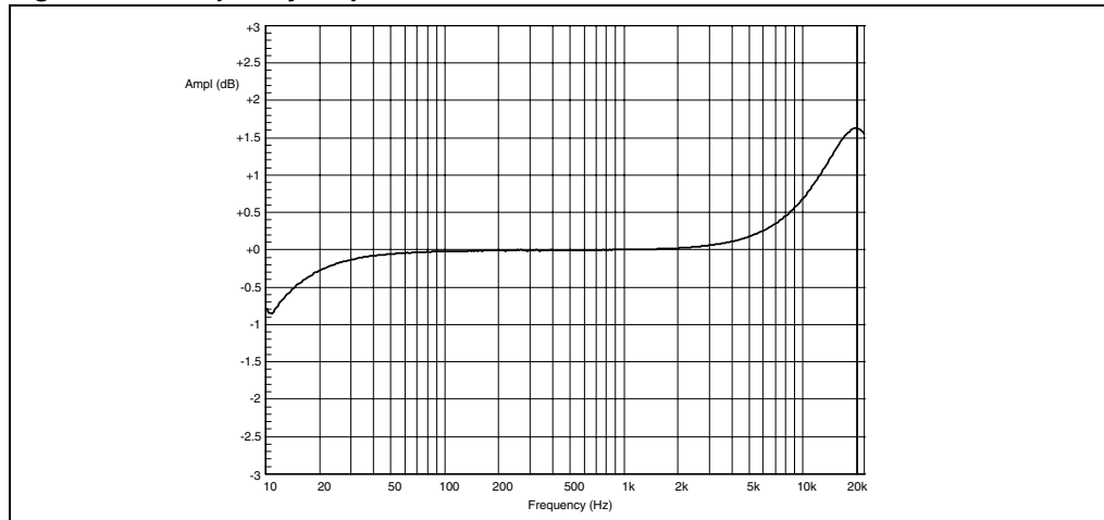
Figure 16. Frequency response
