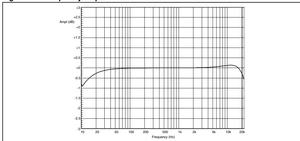
Figure 9. Frequency response
