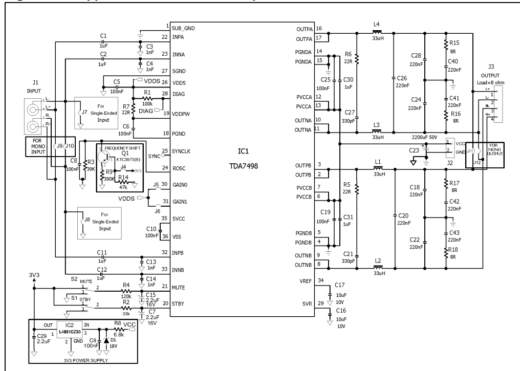
Figure 20. Applications circuit for 8-Ω speakers
