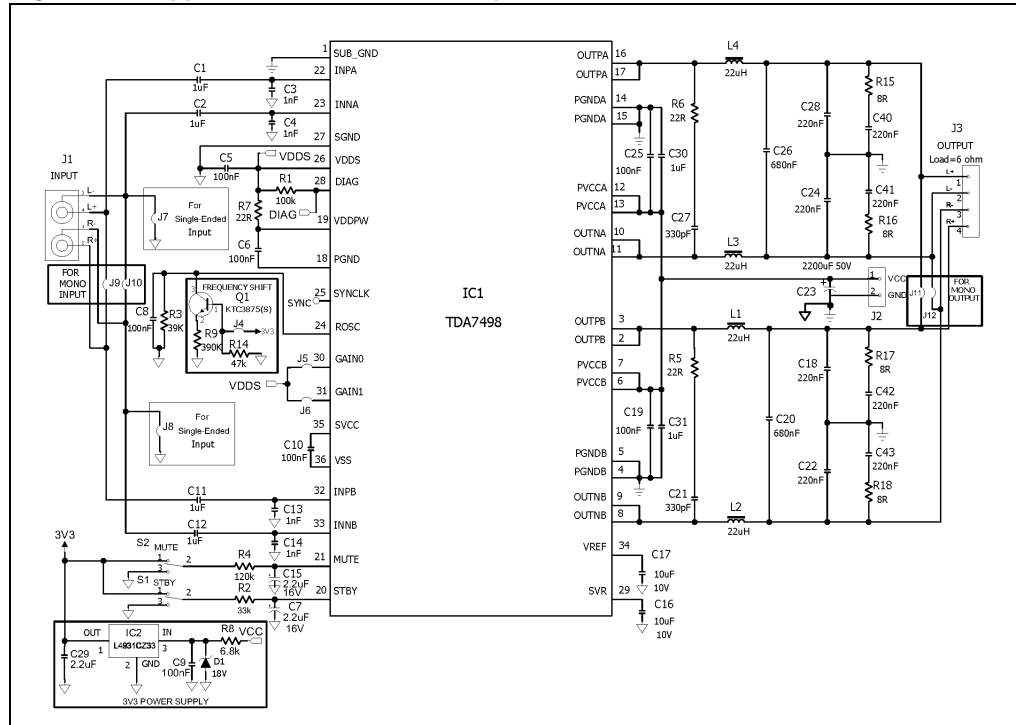
Figure 19. Applications circuit for 6-Ω speakers
