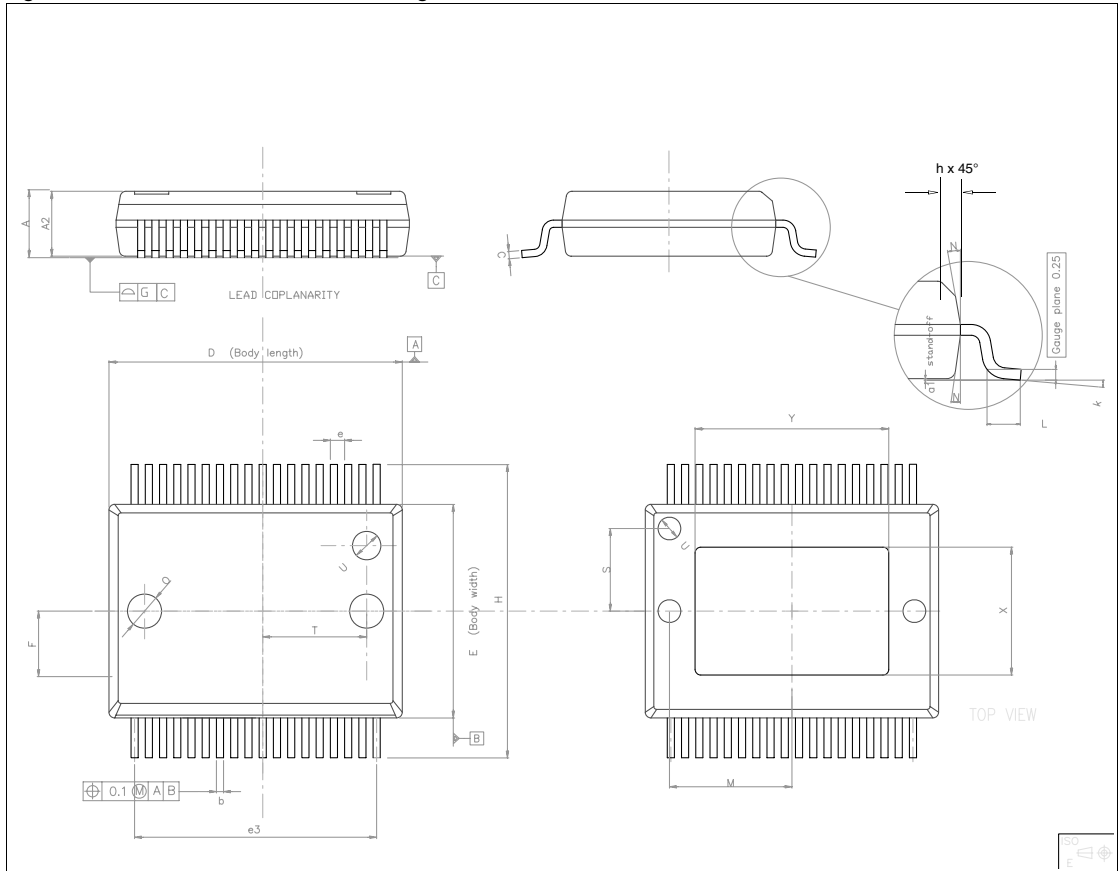
Figure 28. PowerSSO36 EPU outline drawing
