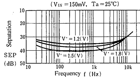
※ Separation vs. Frequency
