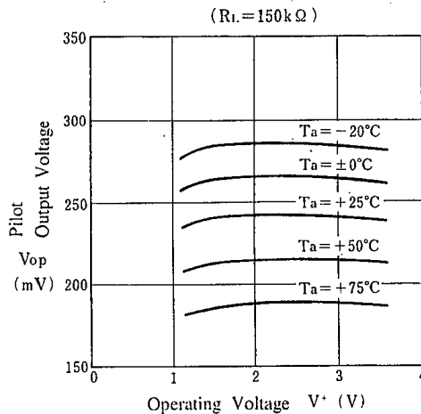
Pilot Output Voltage vs. Operating Voltage
