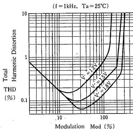
※ Total Harmonic Distortion vs. Modulation
