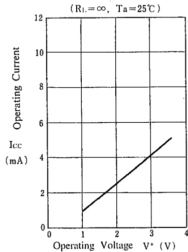
Operating Current vs. Operating Voltage
