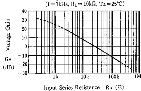
Voltage Gain vs. Input Series Resistance
