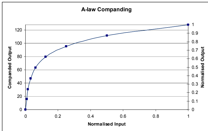
Figure 53 A-Law Companding
