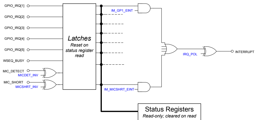
Figure 55 Interrupt Controller
