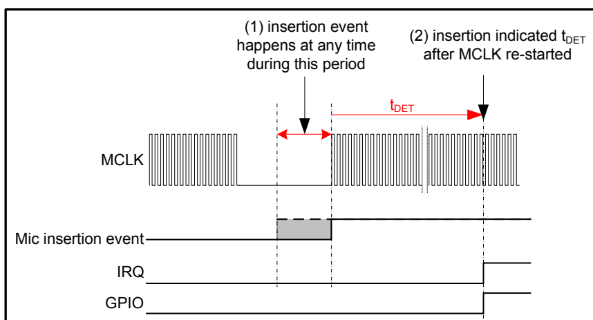
Figure 26 MIC Detection events without MCLK
