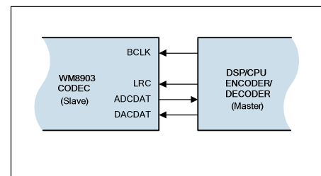
Figure 37 Slave Mode
