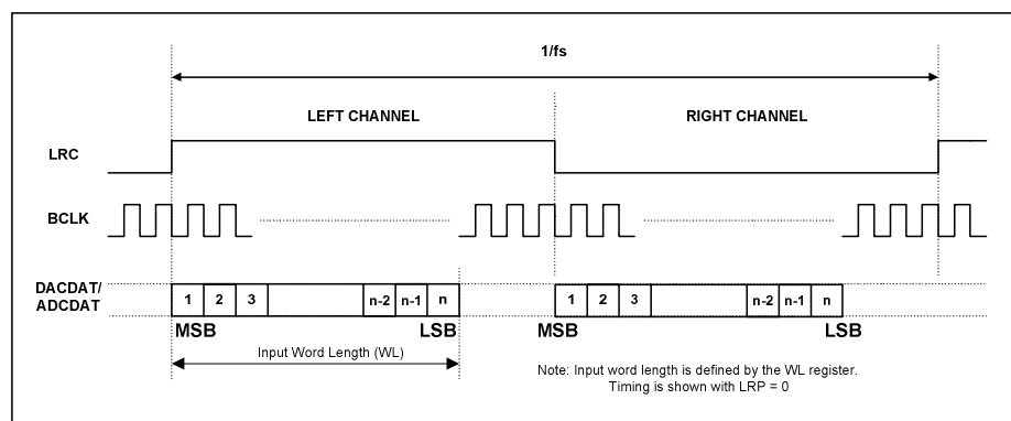
Figure 38 Left Justified Audio Interface (assuming n-bit word length)
