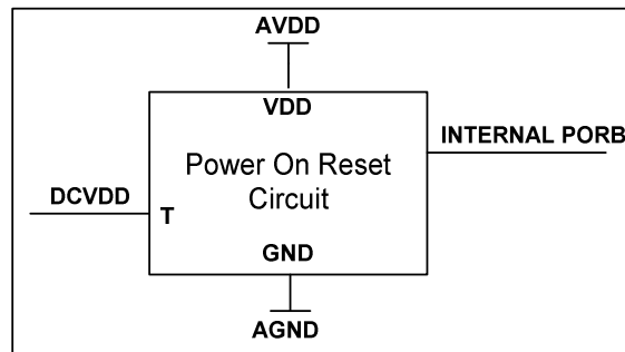
Figure 61 Internal Power on Reset Circuit Schematic
