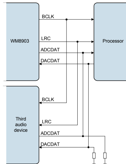
Figure 45 TDM with WM8903 as Master
