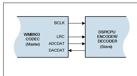
Figure 36 Master Mode
