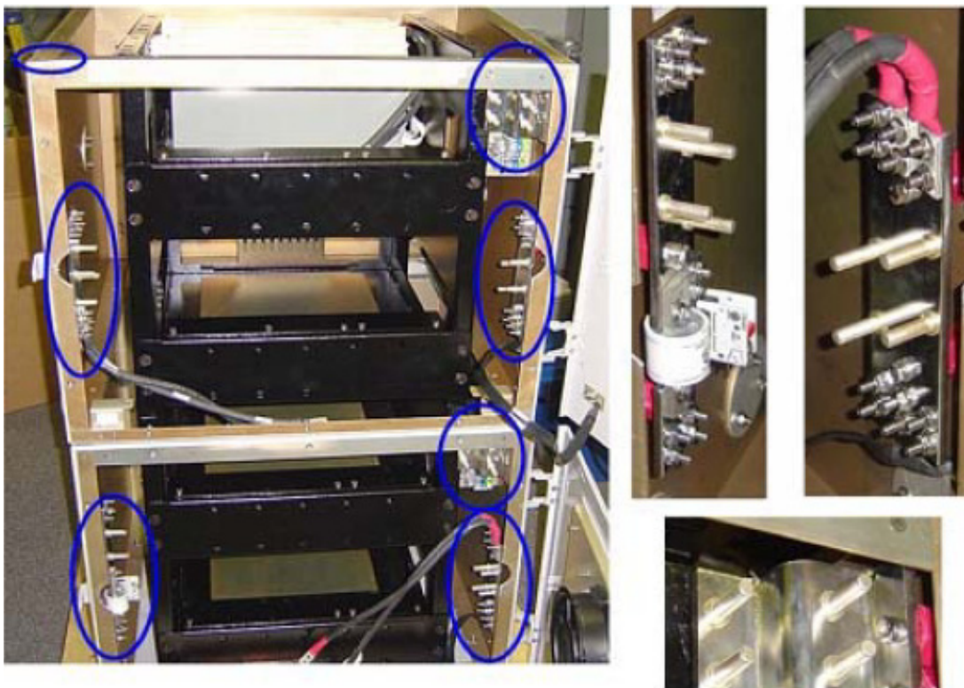
Chassis showing application of Plastic SurLok™
