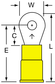
MVU10-6R Stud Size: 6 Wire Range: 12-10
