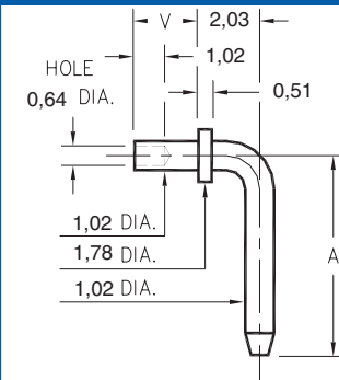
330X-X-14-XX-00-00-08-0 Specify board thickness Swage mount in 1,09 hole
