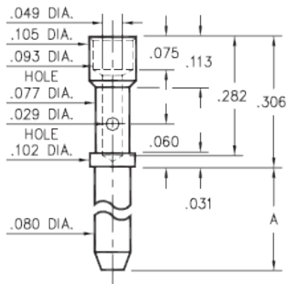
3601-X-07-XX-00-00-08-0 #20A Crimp barrel
